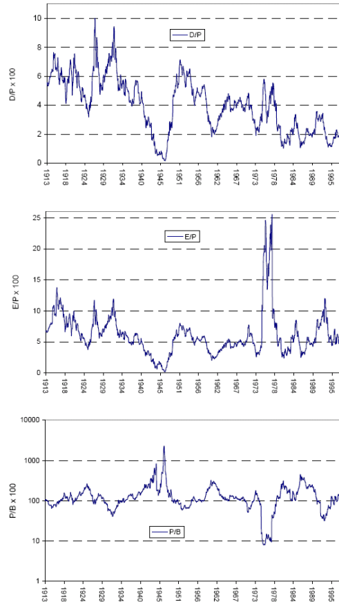
Figure 2: Scaled time series of D/P , E/P , and P/B , 1913-1998
